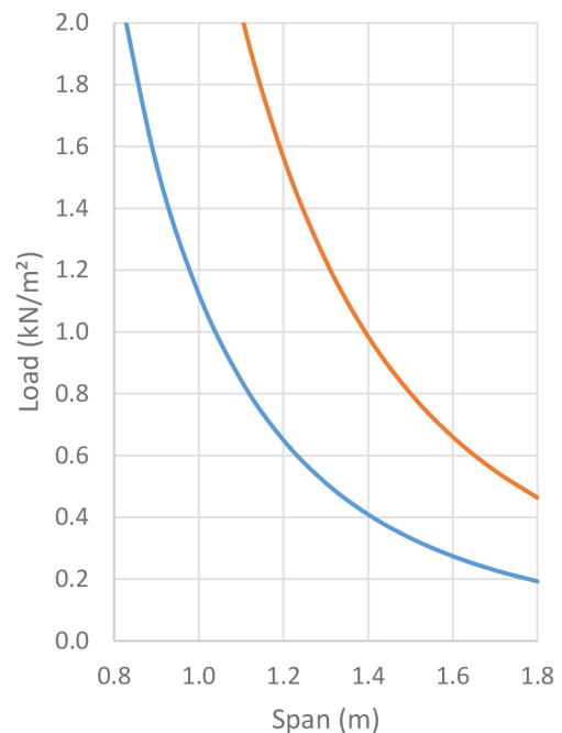
Load/Span
